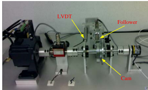
Figure x. Cam mechanism analysis system
